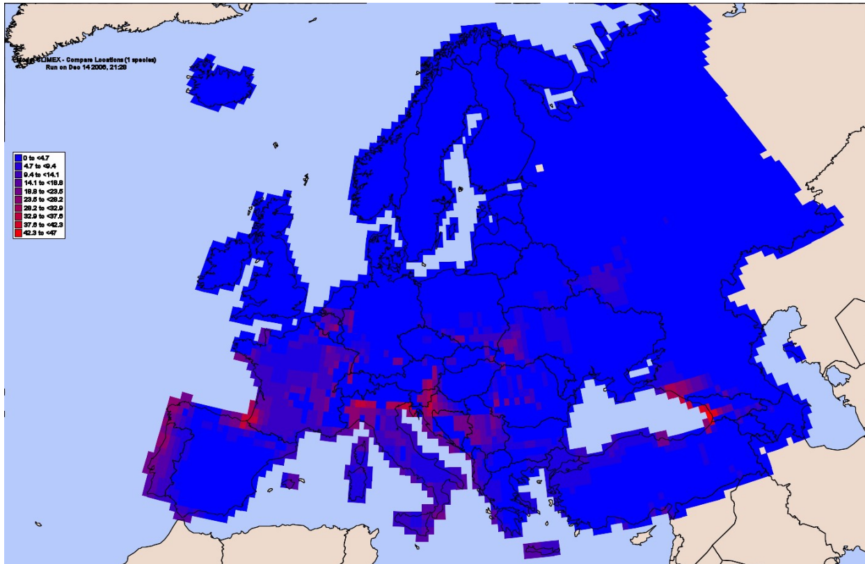
Fig. 12: Polygonum perfoliatum Ecoclimatic Indices for Europe, 30 minutes latitude/longitude resolution (Temperate Template, no cold stress, no wet stress, soil moisture minimum to 0.35, maximum temperature 36°C, DV1=12°C)
